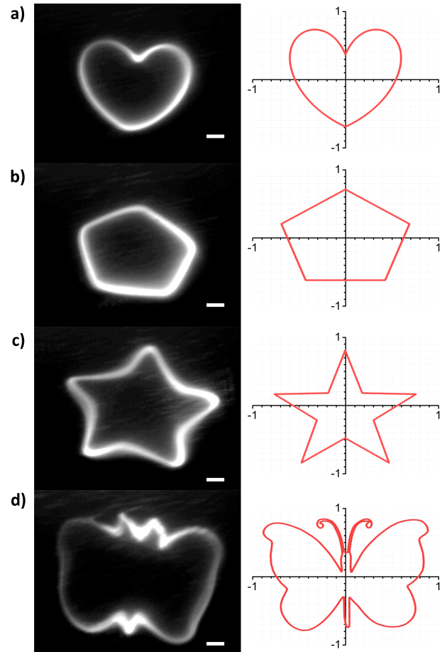
Fig. 4. Free space graphics. Mosaic of images showing the performances of the nanotrap display. On the left side, the image describes the motion of the particle and on the right side the applied trajectory design: (a) heart, (b) pentagon, (c) star and (d) butterfly. We have illuminated the area with a green laser under a diasopic dark-field configuration. The scale bar is 10\mu\text{m} . All the trajectories have been generated under the same conditions: V_{AC}=70\text{ V} , f_{trapping}=4\text{ kHz} , V_{DC}=9\text{ V} , f_{sampling}=100\text{ kHz} . f_{trapping} is the frequency of the applied electrical field while f_{sampling} is the frequency used to scan the points of the particle trajectory. All the images are captured by a coupled objective lens 50\times and a CMOS camera set in POV conditions (50 ms integration time).
