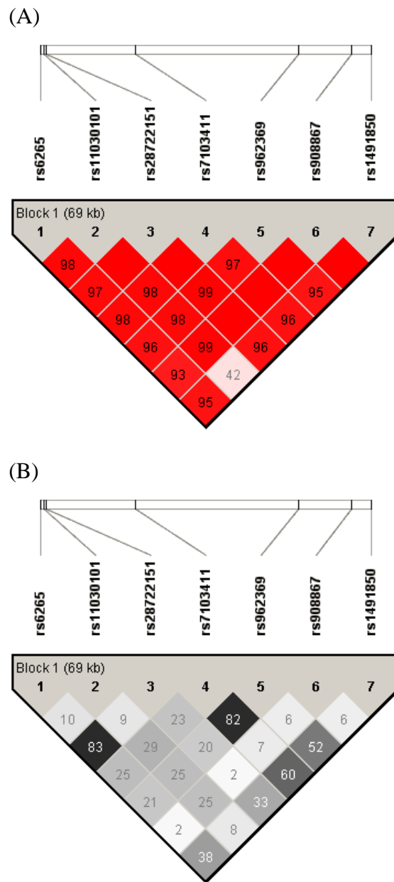
Figure S2. Linkage disequilibrium map of the seven SNPs investigated across BDNF using D' (A) and r^2 (B). The darker the square the higher the correlation.
