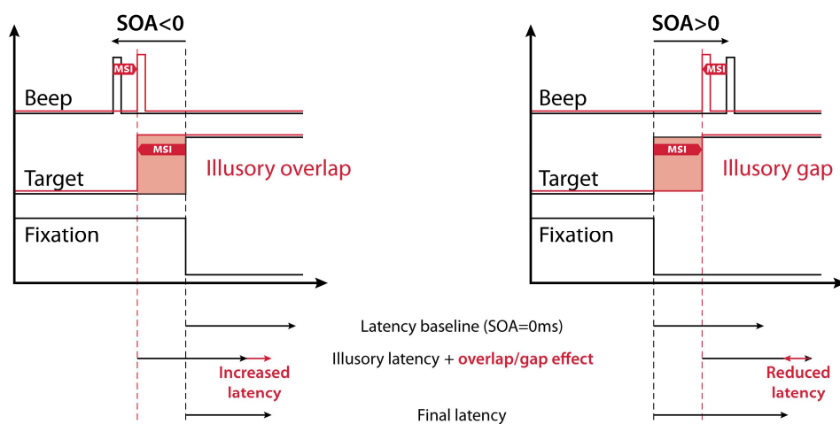
21 Fig 8. Saccade latency components. Illustration of how temporal multisensory integration could 22 introduce an illusory gap/overlap for positive/negative SOA. This additional effect would have reduced 23 the extent of the multisensory modulation of saccade latencies by reducing the effect of the perceived 24 target onset time shift. 25
