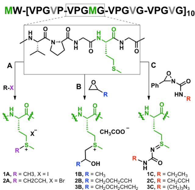
Figure 1. Primary structure of ELP[M 1 V 3 -40] and chemoselective modifications at methionine using alkyl halide (A), epoxide (B) or oxaziridine (C) derivatives. Solvent conditions: A) THF/0.2 M aqu. formic acid; B) AcOH/HFIP (9:1); and C) H 2 O/DMF (99:1).
