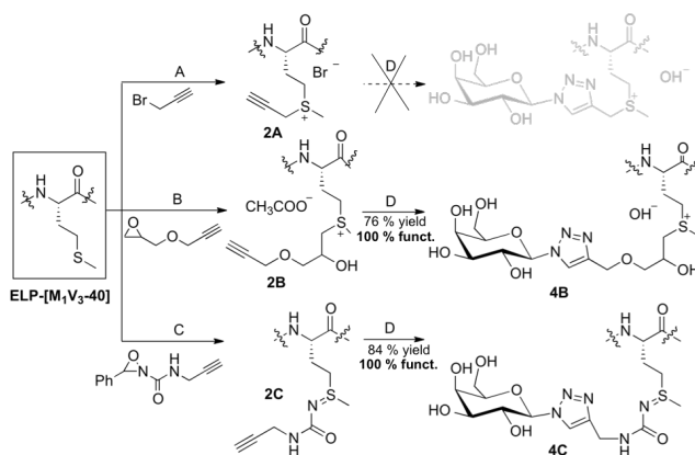
Scheme 1. Synthetic strategies to multivalent galactose-ELP bioconjugates.
