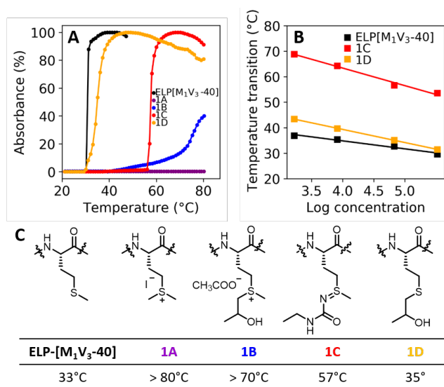
Figure 2. (A) Relative absorbance at 600 nm of ELP[M 1 V 3 -40], 1A, 1B, 1C and 1D at 125 μM in Tris buffer as a function of temperature. (B) T t values of ELP[M 1 V 3 -40], 1C and 1D as functions of concentration in Tris buffer. Lines correspond to the fits of the data using Chilkoti and co-workers empirical equation. 49
