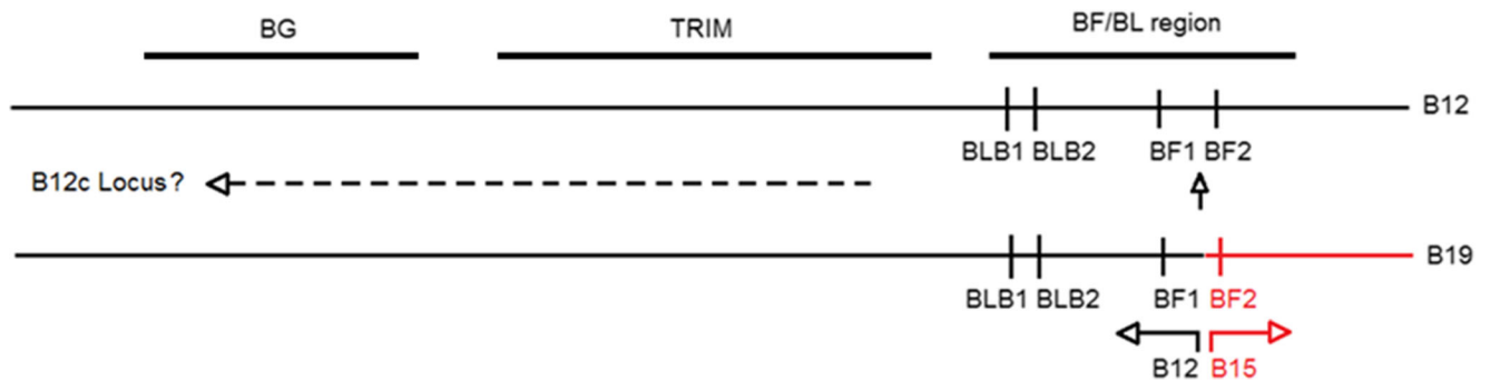
Fig. 8 Inferred location of the third BLB gene by comparison of B12 and B19 haplotypes for the BG, TRIM and BF-BL regions, showing the recombination between the B12 and B15 haplotypes to give the B19 haplotype. Black horizontal line indicates sequence identical (or nearly
