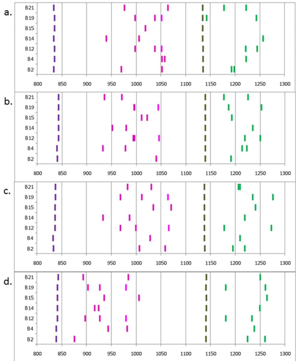
Fig. 7 Chart of migration scores for peaks from samples of haplotype B2, B4, B12, B14, B15, B19 and B21 (from bottom to top) with a FLR combination A (BLB1*1501 and BF2*1501), b FLR combination B (BLB1*0201 and BF1*0201), c FLR combination C (BLB2*0401 and BF2*0401) and d FLR combination D (BLB2*0201 and BF1*0401) based on data in Fig. 6a–d. The migration scores are indicated by lines that are purple for homoduplex peaks and pink for experimental peaks from class II FLRs and dark green for homoduplex peaks and light green for experimental peaks from class I FLRs
