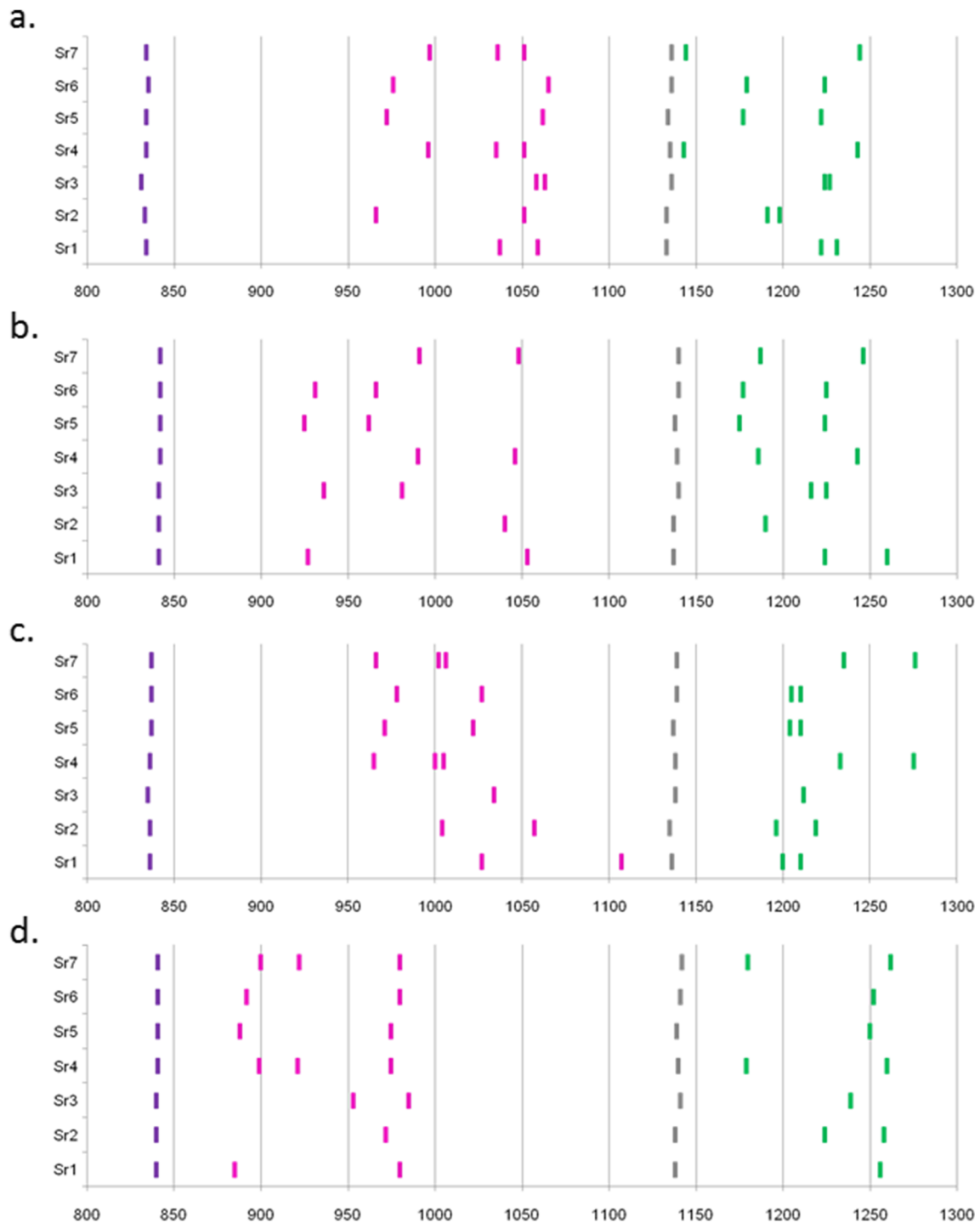
Fig. 9 Chart of migration scores for peaks from samples of French experimental lines corresponding to haplotypes Sr1, Sr2, Sr3, Sr4, Sr5, Sr6 and Sr7 (from bottom to top) with a FLR combination A (BLB1*1501 and BF2*1501), b FLR combination B (BLB1*0201 and BF1*0201), c FLR combination C (BLB2*0401 and BF2*0401) and d
