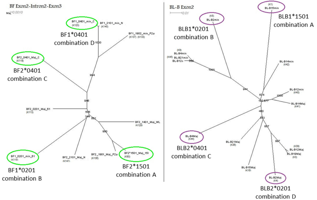
Fig. 4 For both class I and class II B gene sequences, the four most divergent sequences were chosen to make FLRs. Nucleotide sequence alignments of exon 2 to exon 3 from class I (BF1 and BF2) genes (left panel) and of exon 2 from class II B (BLB1 and BLB2) genes (right
