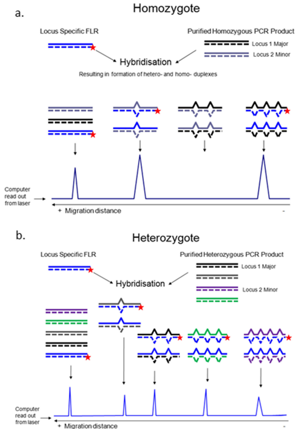
Fig. 1 A diagram representing the four steps of RSCA (amplification to make an FLR, amplification from an experimental sample, hybridization to create DNA duplexes and analysis by capillary electrophoresis) with an idealized trace for a two gene system from a a homozygote (with all possible DNA duplexes shown, including those without an FLR, which would not be detected) and b a heterozygote (with only the DNA duplexes that include an FLR for detection shown). A homozygote sample produces one homoduplex and two heteroduplex peaks in the trace due to the labelled FLR; unlabelled strands form heteroduplexes but are not detected by the machine. A heterozygote sample produces one homoduplex and up to four heteroduplex peaks for a two-locus gene family (BLB or BF), but duplexes between unlabelled DNA strands are not detected (not shown for heterozygote). This figure is based conceptually on Argüello et al 1995
