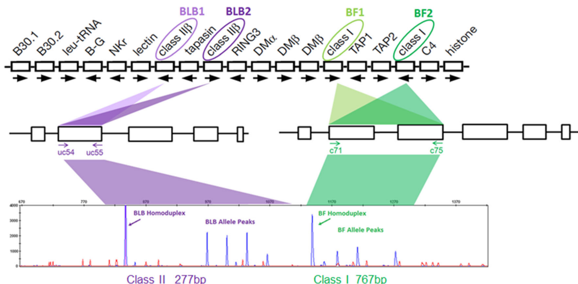
Fig. 2 The genomic basis for simple RSCA typing of chicken classical class I and class II B genes. Top portion shows the BF-BL region, which contains only two BLB and two BF genes (based on Kaufman et al. 1999); middle portion shows intron-exon structures with the location of
