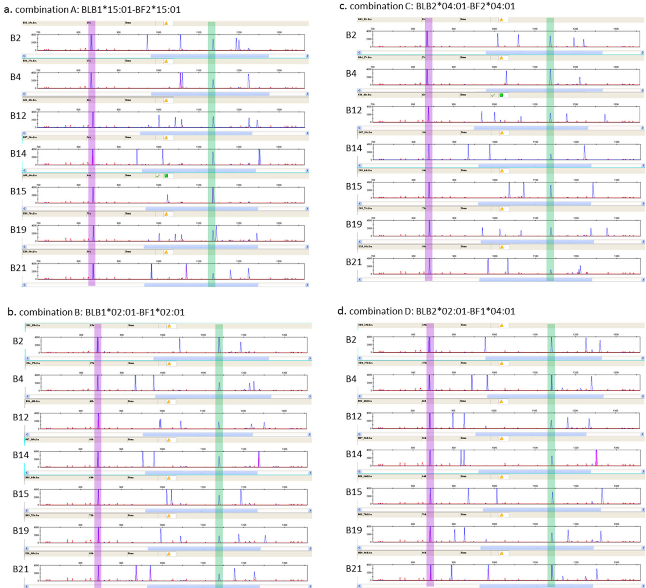
Fig. 6 Examples of RSCA traces from hybridization of genomic DNA from homozygous samples of haplotype B2, B4, B12, B14, B15, B19 and B21 (from top to bottom) with a FLR combination A (BLB1*1501 and BF2*1501), b FLR combination B (BLB1*0201 and BF1*0201), c FLR combination C (BLB2*0401 and BF2*0401) and d FLR combination D
