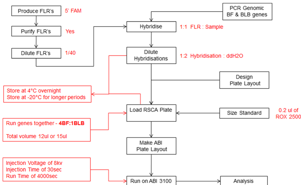
Fig. 3 Work flow for the RSCA experiments described in this report. Each step of the flowchart (as well as several others not shown, some of which are discussed in the text) needed optimization in order to apply the typing method to unknown populations. Red text and boxes indicate the results of optimization steps
