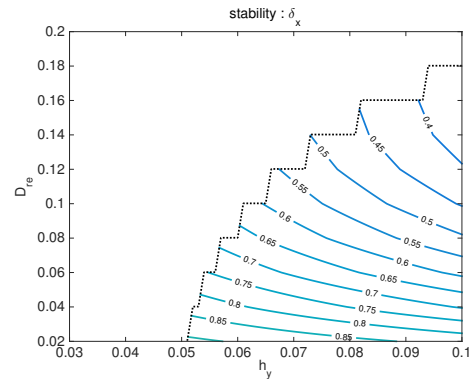
Fig. 6. Stability of the walk for several amplitudes of oscillation h_y and different D_{re} , \delta_X = (h_y, D_{re}) with z = 0.96 - h_y + h_y \cos(3\pi Y) . The black dotted line limits the set of values that corresponds to cyclic motions.
