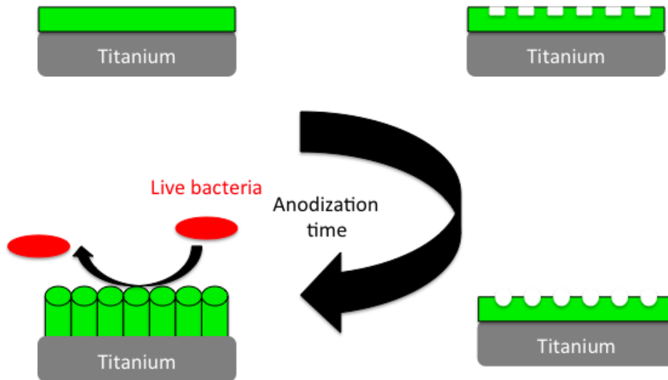
Scheme 3: Formation process of nanotubes on titanium surfaces. Before anodization, a nanoscale \text{TiO}_2 passivation layer is present on Ti surfaces and whenever a constant voltage is applied, pits are formed on the \text{TiO}_2 layer. As anodization time increases, pits grow longer and larger resulting in nanopore formation. After a specific anodization time, nanotubes are formed on the Ti surface.
