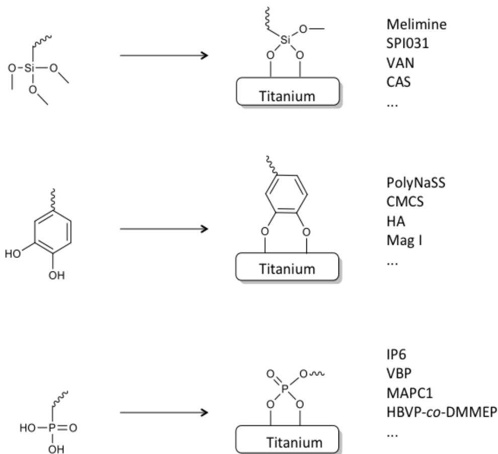
Scheme 2: A selection of anchors on titanium surfaces with different functionalizations to achieve an antimicrobial surface.
