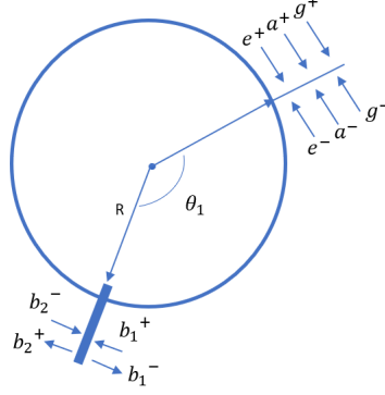
Fig. 3 Waves in an axial-symmetric jointed structure excited by a point load
