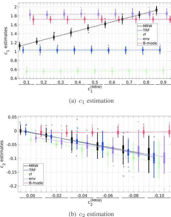
Fig. 4. Average and standard deviation values for estimates of c_1 (for c_2 = -0.06 fixed) and c_2 (for c_1 = 0.5 fixed).
