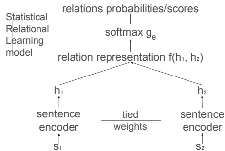
Figure 1: Implicit SRL model in text relation prediction
