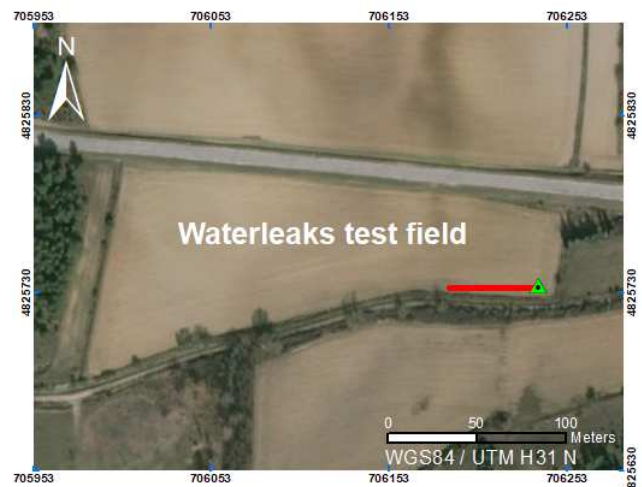
Figure 1: Waterleaks test field. The green mark corresponds to the hydrant. The red line shows the leaking pipeline.
