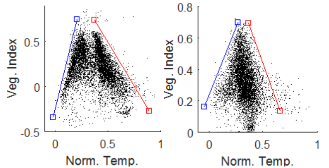
Figure 3: 2D scatterplots of Vegetation Index VI vs. normalized brightness temperature from the manned aircraft (left) and from the UAV (right). The wet edge is in blue and the dry edge is in red.
