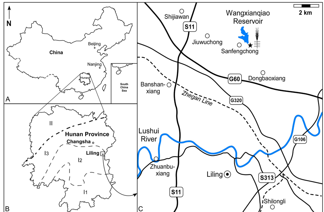
Fig 1. Geographical and geological contexts of the plant-bearing fossil locality. (A) The Hunan Province locates in the South China. (B) The Devonian sediments distribution in Hunan Province. I: Central-Southern Region; I 1 : Jiangyong-Laiyang Unit, I 2 : Shaoyang-Liling Unit, I 3 : Anhua-Liuyang Unit; II: Northwestern Region. (C) The fossil locality of Wangxianqiao Reservoir is close to the Liling City, Hunan Province. Notes: G, National highway; S, Province highway.
