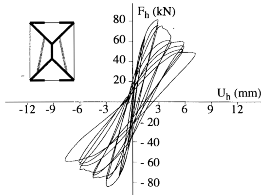
(c) Essai de cisaillement cyclique [1]
