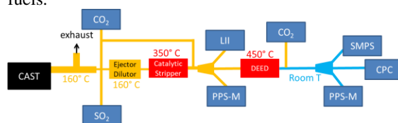
Figure 2. Scheme of the sampling line for Jetscreen tests
