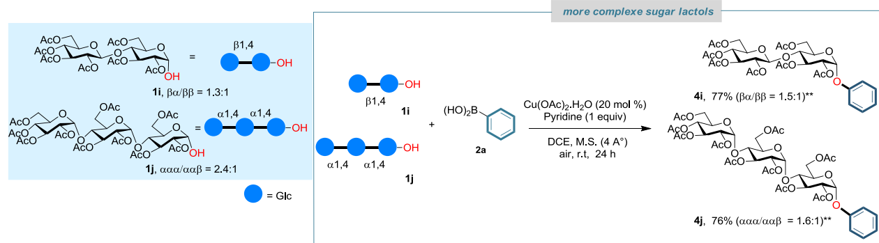
Scheme 3 Scope of the Cu-Catalyzed O -Arylation with more complex carbohydrates a
