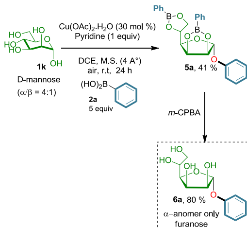
Scheme 4 Cu-catalyzed O -arylation of unprotected \alpha -Man 1k with phenylboronic acid 2a a
