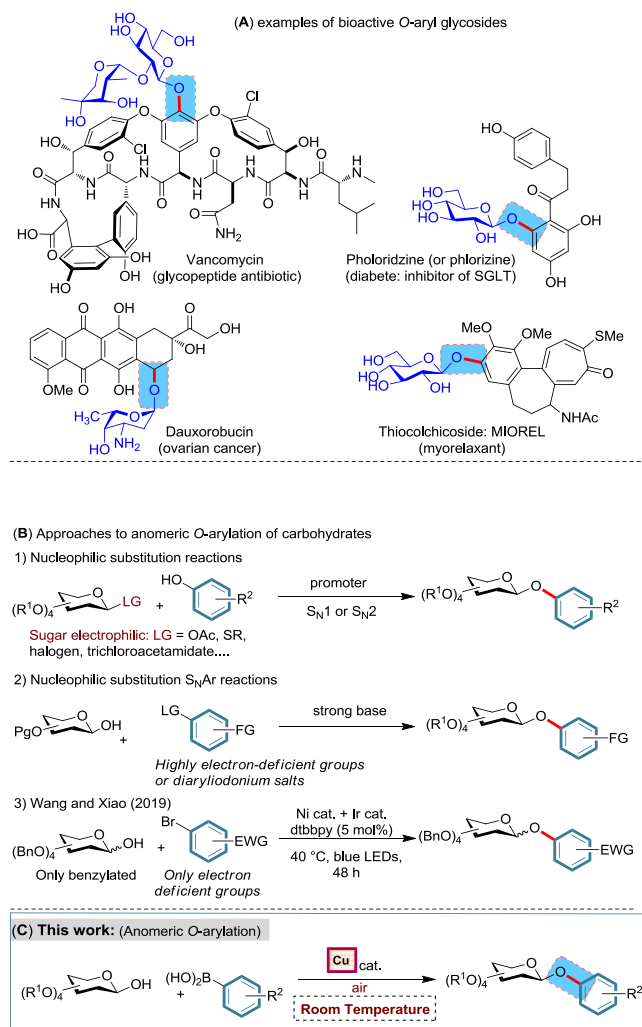
Figure 1. Example of bioactive O -aryl glycosides, and approaches to anomeric O -arylation of carbohydrates
