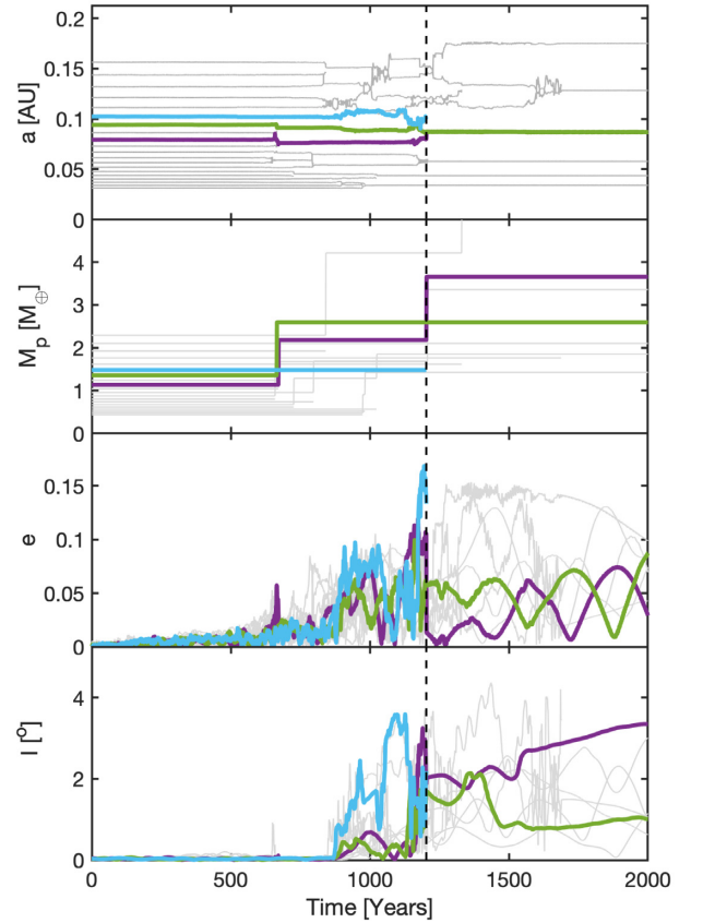
Figure 14. An example of the formation of a co-orbital planet pair by an inelastic collision. Shown are the evolution of the semimajor axes (top panel), planet masses (second panel) eccentricities (third panel), and inclinations (fourth panel). The time interval shown is the first 2000 yr of the simulation, and the collision occurred after \sim 1200 yr (dashed line). The representing three bodies involved in the encounter are marked in blue, green, and purple, where we name them planet-b, planet-g, and planet-p, respectively.
