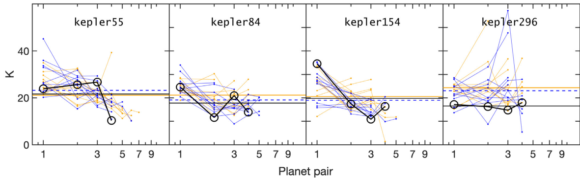
Figure C2. Same plot as Fig. 12 but for the imperfect Kepler55, 84, 154, and 296 templates.
