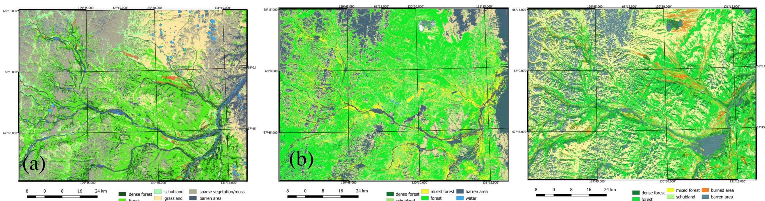
Figure 2. Land cover classification (a) June 2019 (b) July 2019 (c) August 2019
