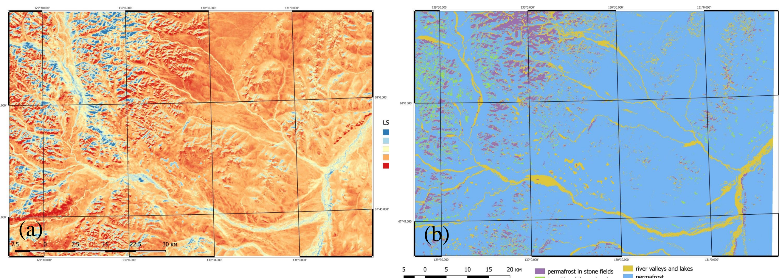
Figure 4. (a) LST Landsat 8 OLI/TIRS July 2019 and (b) Permafrost pattern map
