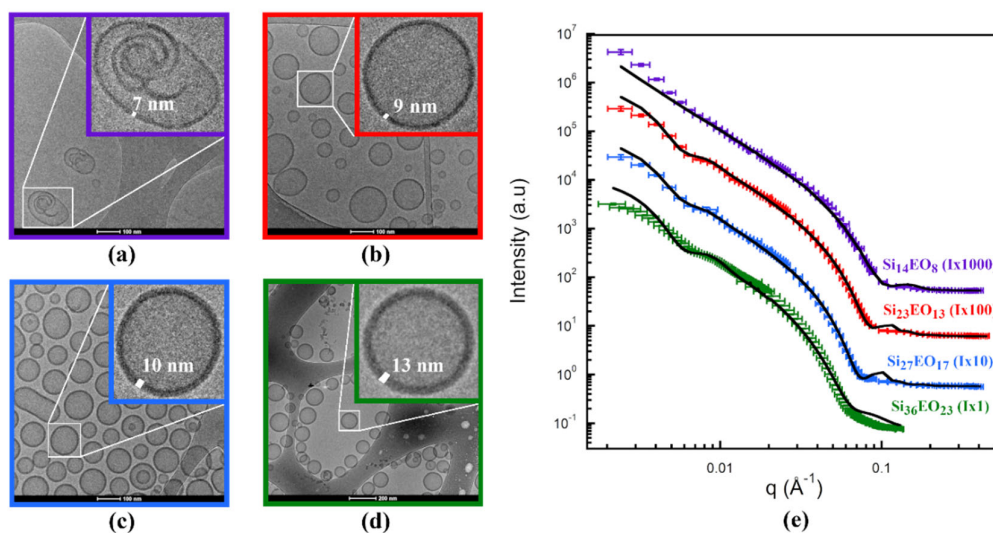
Figure 4. (a–d) Cryo-TEM images of polymersomes obtained for the different copolymers: (a) polymersomes obtained from Si 14 EO 8 ; (b) polymersomes obtained from Si 23 EO 13 ; (c) polymersomes obtained from Si 27 EO 17 ; and (d) polymersomes obtained from Si 36 EO 23 . Inserts show zooms on single polymersomes with the measured membrane thickness. (e) SANS curves of the four diblocks. Black lines represent the best fits using the polydisperse vesicle model.
