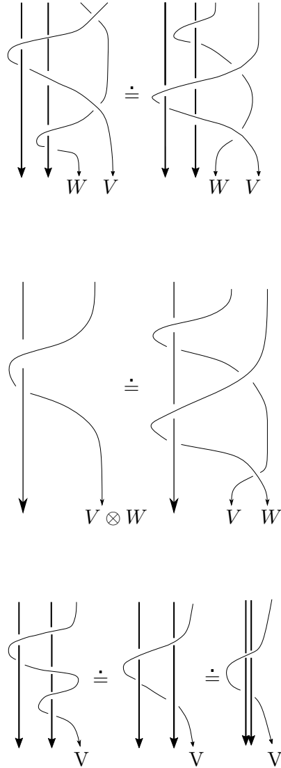
Figure 6.2 : the colored braid identities representing the exchange relation (42) (top), the fusion relation (22) (middle), and the relation (48) (bottom).
