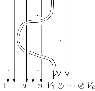
Figure 8.2: a generating morphism of Rib_{n, \mathcal{C}_A} not in Rib_{\mathcal{C}_A} .
