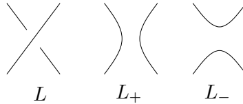
Figure 8.4: skein related ribbon links.
