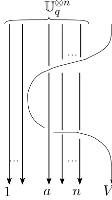
Figure 6.1 : the colored braid representing (id \otimes \Phi_n)(M^{(a)}) .
