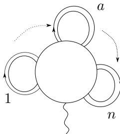
Figure 1.1 : the daisy graph
