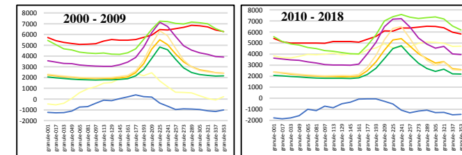
Figure 7 : variations in chlorophyll activity of differents types of vegetation
