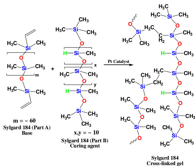
Figure 1 The chemical structure of Sylgard®184 elastomers [31]
