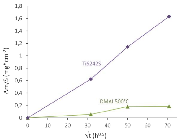
Fig. 6. Mass gain per unit area for bare and coated Ti6242S coupons as a function of the square root of annealing time at 600°C.
