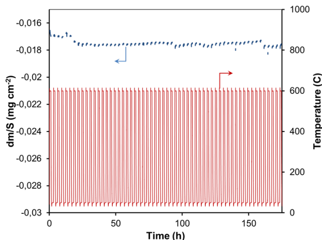
Fig. 7. Evolution of the mass gain per unit area of a sample coated at 300 °C, and of the temperature variation (cycling) as a function of time.
