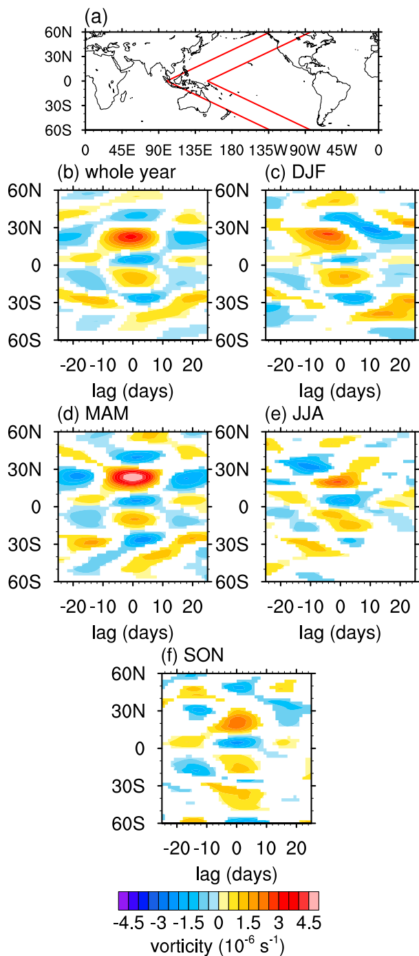
FIG. 15. Slanted time–latitude sections of the lag-regressed vorticity ( \times 10^{-6} \text{ s}^{-1} ) against the third local PC. (a) The longitude range is marked by the red lines. The regression is for (b) the whole year, (c) DJF, (d) MAM, (e) JJA, and (f) SON. Only values above the 99% confidence level are shown.
