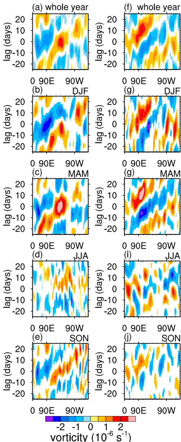
FIG. 16. Time–longitude sections of the lag-regressed vorticity ( \times 10^{-6} \text{ s}^{-1} ) against the third local PC for (a),(f) the whole year, (b),(g) DJF, (c),(h) MAM, (d),(i) JJA, and (e),(j) SON, averaged over (a)–(e) 20^{\circ} – 35^{\circ}\text{N} and (f)–(j) 20^{\circ} – 35^{\circ}\text{S} . Only values above the 99% confidence level are shown.
