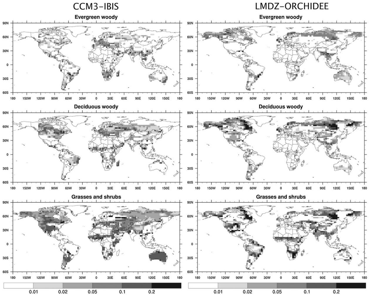
FIG. 2. Standard deviation of the mean foliage projected cover simulated by (left) CCM3-IBIS and (right) LMDz-ORCHIDEE, for (top) evergreen trees, (middle) deciduous trees, and (bottom) grasses plus shrubs.
