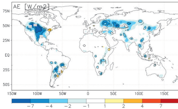
FIG. 10. Mean annual LULCC-induced change in available energy, averaged over all models and all experiments [ 0.5(\text{PD} - \text{PD}_v + \text{PI}_v - \text{PI}) ]. Shadings refer to the changes in \text{W m}^{-2} , while isolines represent the standard deviation between the models.
