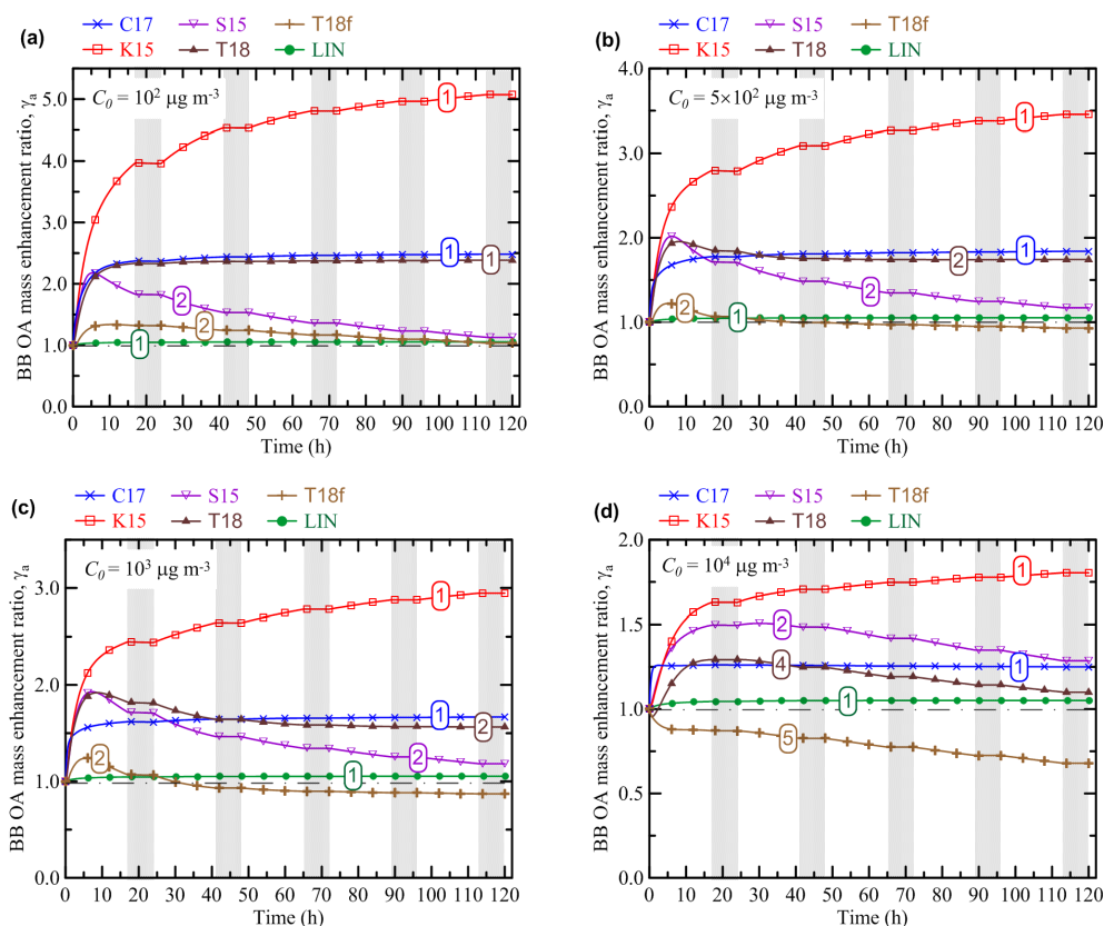
Figure 3. Evolution of the BB OA mass enhancement ratio ( \gamma_a ) according to the simulations performed with the different OA schemes and with different values of the initial mass concentration of BB OA: (a) C_0 = 10^2 \mu\text{g m}^{-3} , (b) C_0 = 5 \times 10^2 \mu\text{g m}^{-3} , (c) C_0 = 10^3 \mu\text{g m}^{-3} , and (d) C_0 = 10^4 \mu\text{g m}^{-3} . The initial BB plume size, S_p , was fixed at 5 km in all the simulations shown. Shaded bands depict nighttime periods when no oxidation reactions were allowed to occur. The numbers on the curves denote the different dynamical regimes of BB OA evolution according to the definitions in Sect. 3.1. A horizontal dashed–dotted line in each panel indicates the situation where no BB OA mass enhancement occurs ( \gamma_a = 1 ).
