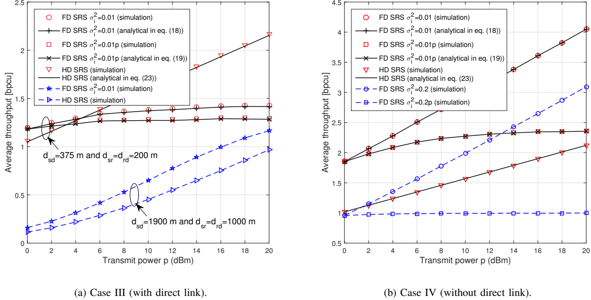
Fig. 3: Throughput with transmit power of Model II for FD and HD when K = 3 and N = 4 .
