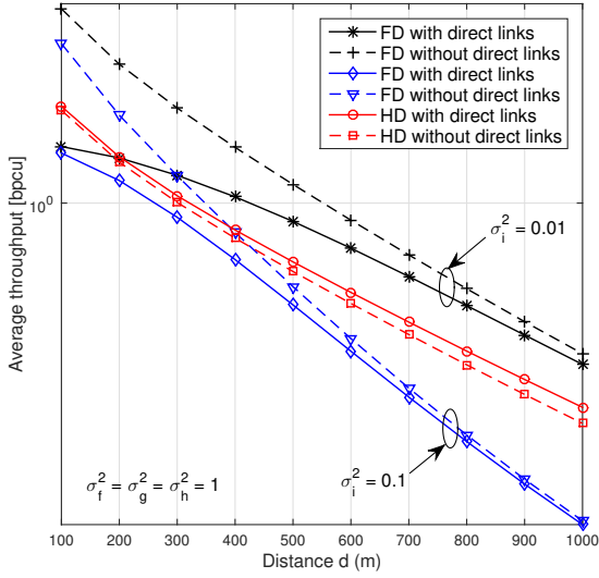
(a) With distance ( l_{sr} = l_{rd} = d and l_{sd} = 1.9d ).
