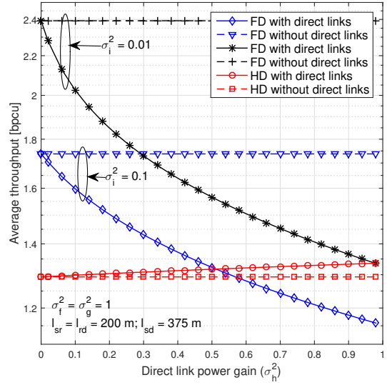
(b) With variance \sigma_h^2 .
