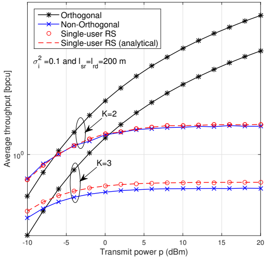
(a) Orthogonal/non-orthogonal transmission.
