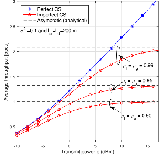
(b) Perfect/imperfect CSI ( K = 3 ).
