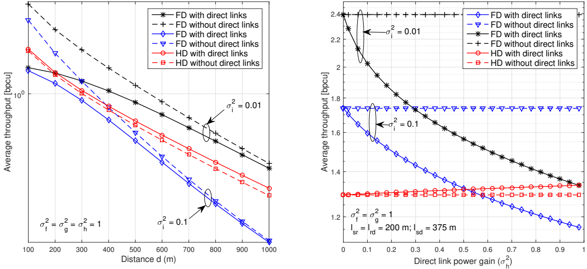
(a) With distance ( l_{sr} = l_{rd} = d and l_{sd} = 1.9d ).
