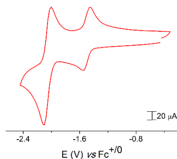
Figure 2 Cyclic voltammogram of complex 1 recorded at 1 V \text{s}^{-1} with glassy carbon as working electrode in ACN and 0.1 M n\text{Bu}_4\text{NPF}_6 supporting electrolyte.
