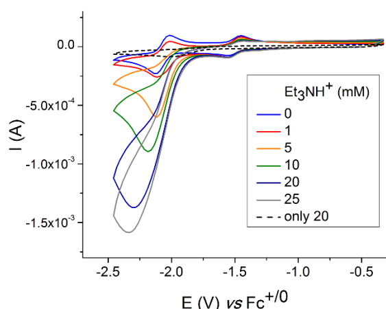
Figure 5 Cyclic voltammograms of complex 1 (1 mM) with increasing amounts of \text{Et}_3\text{NH}^+ (1–20 mM) in ACN (0.1 M n\text{Bu}_4\text{NPF}_6 glassy carbon working electrode) at 30 \text{ V s}^{-1} . The dotted line is obtained at 20 mM of \text{Et}_3\text{NH}^+ in the absence of complex 1 .
