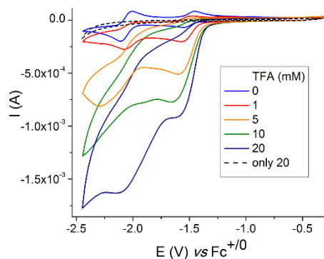
Figure 3 Cyclic voltammograms of complex 1 (1 mM) with increasing amounts of TFA (1–20 mM) in ACN (0.1 M n\text{Bu}_4\text{NPF}_6 , glassy carbon working electrode) at 30 V \text{s}^{-1} . The dotted line is obtained at 20 mM of TFA in the absence of complex 1 .
