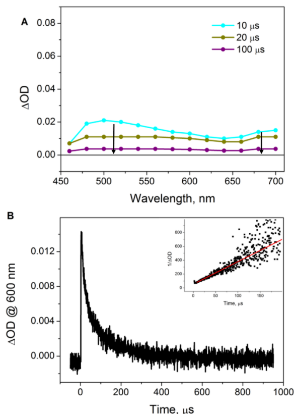
Figure 7 Laser flash photolysis experiments (excitation at 532 nm) of \text{N}_2 -purged solutions containing 50 \mu\text{M} \text{Ru}(\text{bpy})_3\text{Cl}_2 \cdot 6\text{H}_2\text{O} , 0.1 M ascorbic acid, and 0.1 mM 2 in 1 M acetate buffer (pH 4): A) Spectral evolution between 10-100 \mu\text{s} ; B) kinetic trace at 600 nm; (inset) second-order kinetic treatment for the estimation of the bimolecular rate constant.
