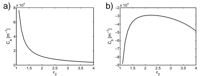
Fig. 9. Coupling coefficients C_a and C_b as function of \varepsilon_2 , when \varepsilon_1 = 1.0 . Solid lines represent values calculated with classic CMT model (Eq.(8)); dotted lines represent values C'_a(\varepsilon_2) + C''_a(\varepsilon_2) and C'_b(\varepsilon_2) + C''_b(\varepsilon_2) , where C'_a(\varepsilon_2) , C''_a(\varepsilon_2) , C'_b(\varepsilon_2) and C''_b(\varepsilon_2) are approximated by Eq.(17) and Eq.(18) after calculation of C'_a(\varepsilon_1) , C''_a(\varepsilon_1) , C'_b(\varepsilon_1) and C''_b(\varepsilon_1) . Wavelength is 750 nm. a) C_a ; b) C_b
