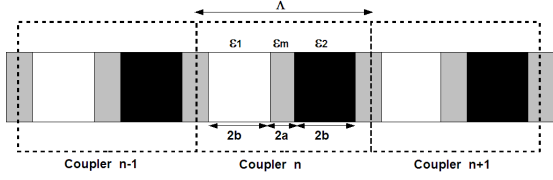
Fig. 1. The plasmonic array studied in this paper. Two cores with dielectric constant \varepsilon_1 and \varepsilon_2 (white and black respectively) are alternated and divided by a metal layer (grey) whose dielectric constant is \varepsilon_m . Width of cores is 2b , width of metal layers is 2a . The fundamental period \Lambda is 4a + 4b . Dashed rectangles surround 3 consecutive basic cells of the array, that according to the CMT developed in this paper are plasmonic couplers.
