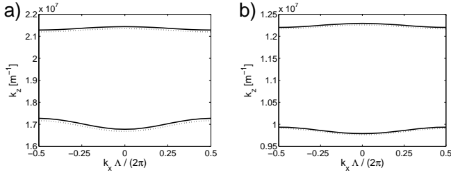
Fig. 10. Diffraction curves k_z(k_x) of the non uniform array with 2a = 40nm , 2b = 120nm , \epsilon_1 = 1.0 , \epsilon_2 = 1.5 . k_x is normalized respect to the period \Lambda of the array. Solid line for numerically calculated values; dotted lines for CMT. a) 750 nm; b) 450 nm.
