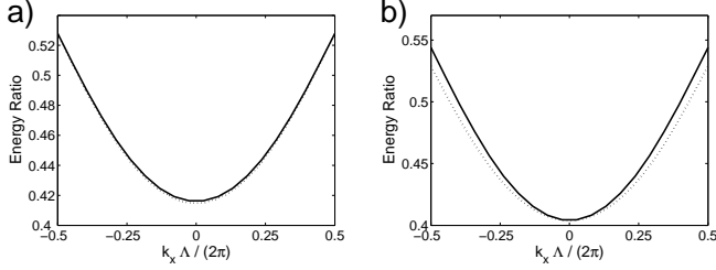
Fig. 11. Ratio En_1/(En_1 + En_2) as function of tilt k when 2a = 40nm , 2b = 120nm , \epsilon_1 = 1.0 , \epsilon_2 = 1.5 . Solid line, numerically calculated values; dotted lines, predicted values (CMT). a) 750 nm; b) 450 nm.
