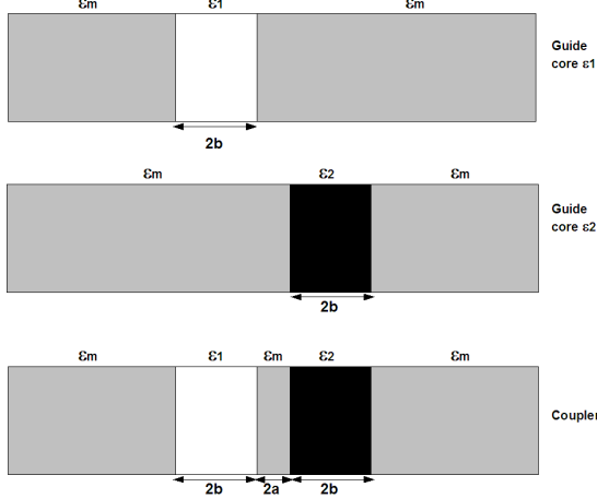
Fig. 2. In the upper and in the center figure two single plasmonic guides are shown. The cores (width 2b ) have dielectric constant \varepsilon_1 and \varepsilon_2 respectively, and are surrounded by metal with dielectric constant \varepsilon_m . In the lower figure there is the coupler used as basic cell in the CMT developed in this paper. Two cores (width 2b ) with dielectric constant \varepsilon_1 and \varepsilon_2 , and divided by a metal layer (width 2a , dielectric constant \varepsilon_m ), are surrounded by metal.
