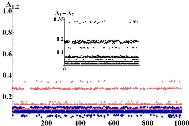
FIG. 4: (Color online) \Delta_1 (light red triangles) and \Delta_2 (dark blue circles) evaluated for 1000 randomly generated bipartite states, with d_M = d_m + 70 and d_m randomly chosen in [2, 5] . For these strongly unbalanced bipartitions we always detect \Delta_1 > \Delta_2 . The inset shows the difference \Delta_1 - \Delta_2 .
