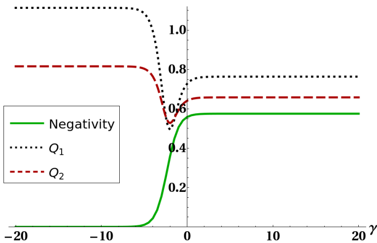
FIG. 6: Negativity of reduced state of the two ultracold atoms (full line), bound Q_1 (dotted line) and bound Q_2 (dashed line) versus quadratic interaction parameter \gamma . The other parameters have been fixed as k_B T = 2 , \tau = 3 , and k = 1 .
