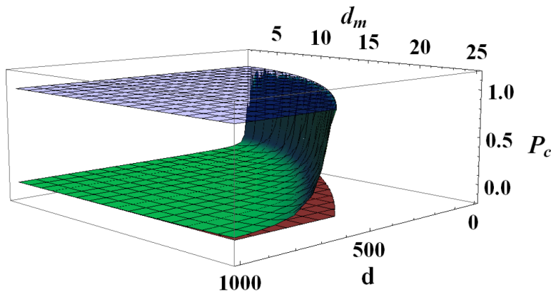
FIG. 1: (Color online) Purity threshold P_c given in Eq. (20) (green surface) and natural purity limits 1 (blue upper surface) and \frac{1}{d} (red lower surface) as functions of d \in [4, 1000] and d_m \in [2, 25] such that d_m^2 \leq d . Values of purity below the green surface are such that Q_1 < Q_2 , while values of purity above the green surface yield Q_2 < Q_1 . It is clear that, when d_m^2 < d , P_c \sim \frac{1}{d} meaning that Q_2 < Q_1 for most of quantum states. On the other hand, when d_m^2 \sim d and Q_1 < Q_2 almost everywhere in state space.
