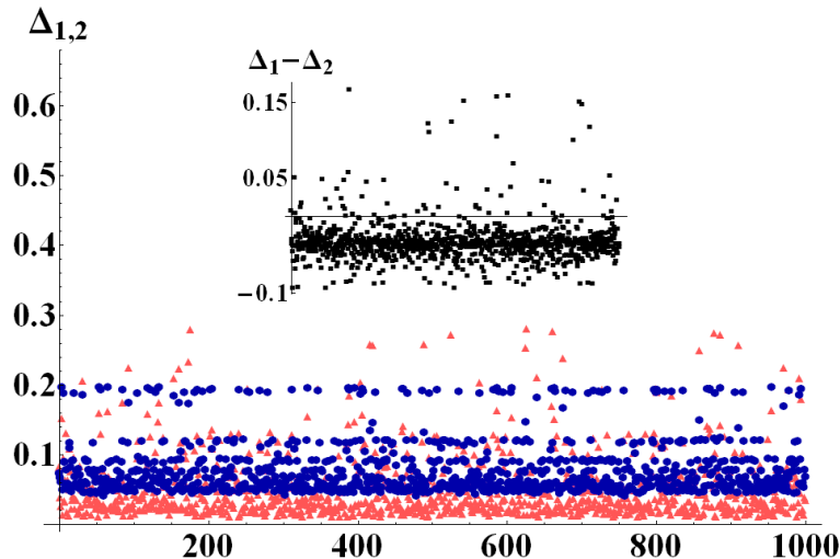
FIG. 3: (Color online) \Delta_1 (light red triangles) and \Delta_2 (dark blue circles) evaluated for 1000 randomly generated bipartite states, with d_M = d_m + 60 and d_m randomly chosen in [2, 10] . Since the bipartitions are no longer perfectly balanced, there is a much broader mixing of values of \Delta_1 and \Delta_2 . In particular, \Delta_1 has a much wider distribution of values, while \Delta_2 seems to have a much denser distribution around central values. The inset shows the difference \Delta_1 - \Delta_2 .
