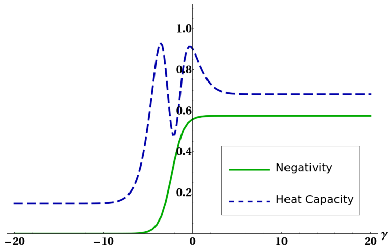
FIG. 5: Negativity of reduced state of the two ultracold atoms (full line) and Heat Capacity of the system (dashed line) versus quadratic interaction parameter \gamma . The other parameters have been fixed as k_B T = 2 , \tau = 3 , and k = 1 .
