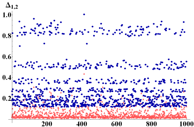
FIG. 2: ((Color online) \Delta_1 (light red triangles) and \Delta_2 (dark blue circles) evaluated for 1000 randomly generated bipartite states, with d_m = d_M randomly chosen in [2, 10] . For these perfectly balanced bipartite states \Delta_1 < \Delta_2 everywhere in state space.
