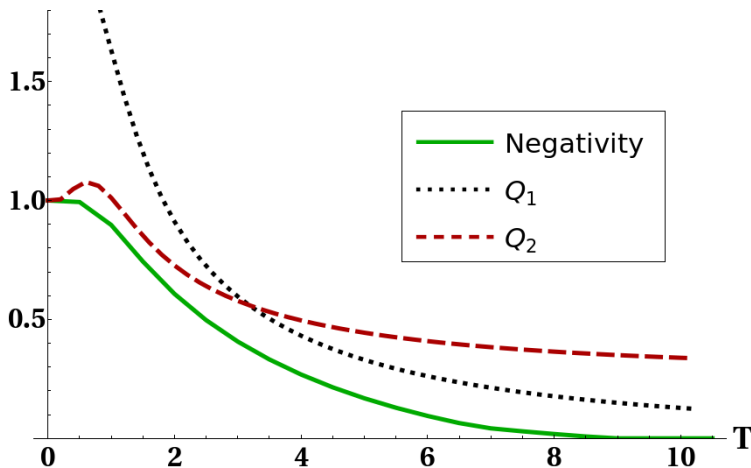
FIG. 8: Negativity of reduced state of the two ultracold atoms (full line), bound Q_1 (dotted line) and bound Q_2 (dashed line) versus temperature T (in units of k_B ). The interaction parameters have been fixed as \tau = 4 , k = 5 and \gamma = 1 .
