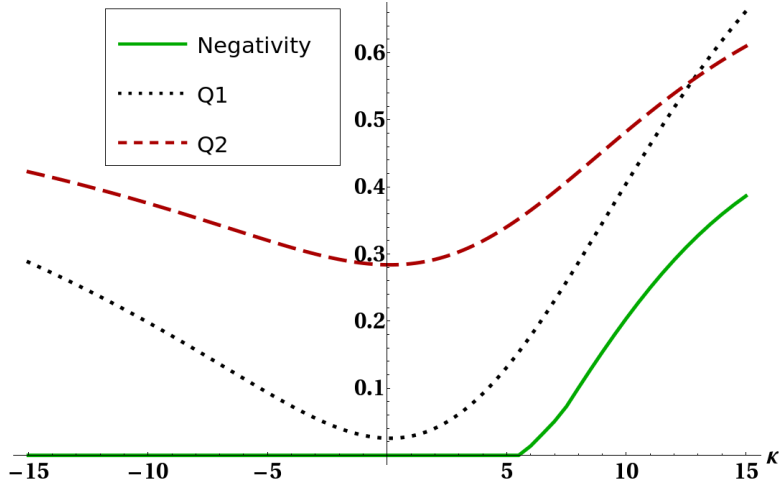
FIG. 7: Negativity of reduced state of the two ultracold atoms (full line), bound Q_1 (dotted line) and bound Q_2 (dashed line) versus Heisenberg interaction parameter k . The other parameters have been fixed as k_B T = 10 , \tau = 3 , and \gamma = 1 .
