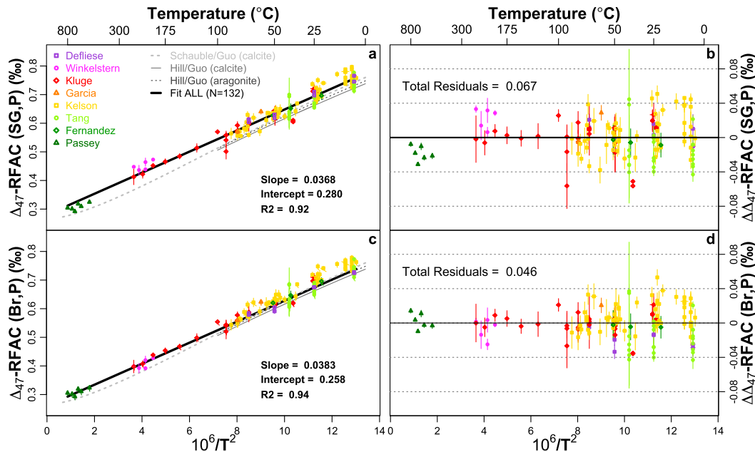
Figure 4. Composite calibration line (Monte Carlo fit) through sample mean \Delta_{47}\text{-RFAC} values (a/c) and offset from corresponding composite calibration ( \Delta_{47}\text{-RFAC} ; b/d), selecting synthetic carbonates only, processed using either Santrock/Gonfiantini (SG) (a/b) or International Union of Pure and Applied Chemistry (IUPAC) (c/d) parameters, new \Delta_{47}\text{-TE} values (Petersen, P, this study) and new \Delta^*_{25-X} values (this study). Error bars represent 1SE external error on the sample mean \Delta_{47} (vertical) or reported error in formation temperature (horizontal). Colors correspond to study, with first author name listed in corresponding color (more details given in Table 1). Theoretical predictions of clumping in solid calcite by Schauble et al. (2006) and calcite and aragonite by Hill et al. (2014) combined with experimentally or theoretically determined fractionation between solid calcite or aragonite, respectively, and \text{CO}_2 from Guo et al. (2009) updated to the absolute reference frame ( \Delta^*_{\text{calcite}} = +0.232 becomes +0.268\text{‰} , \Delta^*_{\text{aragonite}} = +0.229\text{‰} becomes +0.264\text{‰} using Table 4 of Dennis et al., 2011) shown for comparison, although these inherently include an estimation of \Delta^*_{25-X} that has not been updated to IUPAC parameters. This would only differ by 0.004\text{‰} if updated using \Delta^*_{\text{dolomite90}} from Bonifacie et al. (2017) and our +0.088\text{‰} \Delta^*_{25-90} value (Table 2). Linear fit through all data calculated using Monte Carlo sampling approach, with statistics and fit parameters listed in Table 2 and shown in lower right of panels (a) and (c). Total residuals are calculated as the sum of the square of the absolute value of the offset between observed and predicted from the synthetic composite calibration.
