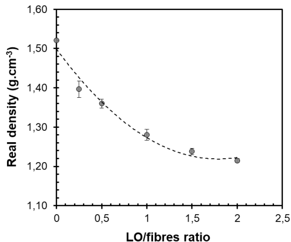
Fig. 4: Density of the coated fibres versus LO/fibre ratio.
