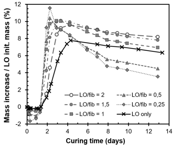
Fig. 3: Mass monitoring of fibres treated with linseed oil during the treatment cure.
