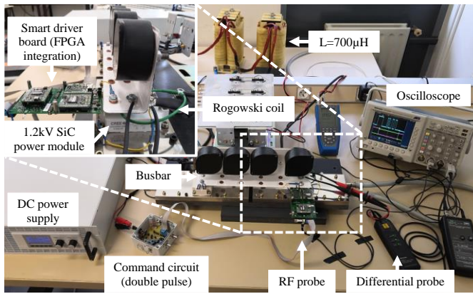
Fig. 14. Experimental setup for evaluation under real switching conditions
