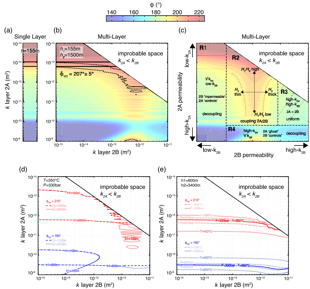
Figure 2. Controls on the phase lag between vent temperatures and M2 tides. (a) In a single layer (2A) of thickness 155 m, a phase lag of 207^\circ requires a permeability of \sim 10^{-13} m 2 (thick contours). (b) By contrast, in a two-layer model of total thickness 1,500 m, the same phase lag requires a specific combination of layers 2A and 2B permeabilities. The two-layer model asymptotes the single-layer model as k_{2B} decreases. (c) Typical phase lag map illustrating the four key regimes (R1–R4) described in section 2.3. (d) Sensitivity of 2 phase lag contours ( 210^\circ in red and 160^\circ in blue) to changes in the thickness of the layers. (e) Sensitivity of the same contours to changes in the assumed average pressure and temperature that set the thermodynamic properties of the fluid in both layers (see section 2.3).
