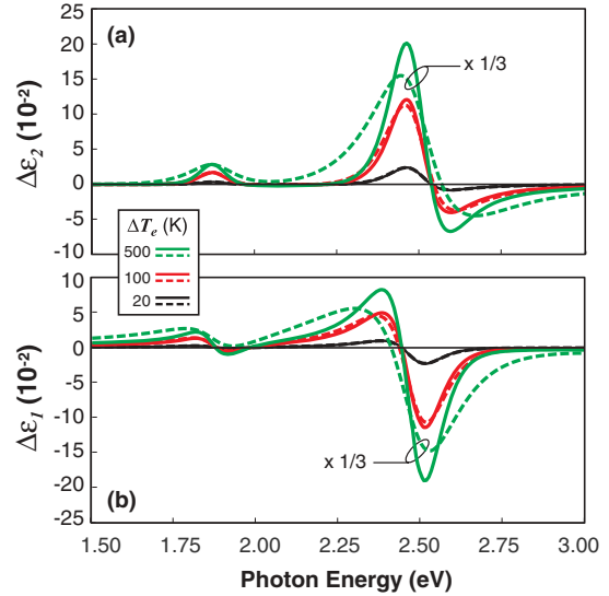
FIG. 2. (Color online) Spectral variation of the (a) imaginary part and (b) real part of the interband dielectric function of gold for three different values of \Delta T_e , computed from Eqs. (11)–(13). Linearized temperature dependence provided by Eq. (13) (solid lines) is compared with exact solution (dashed lines).
