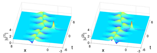
FIG. 4 (color online). As in Fig. 1, with f = 0.1i , a_1 = 1.2 , a_2 = 1.2 .
