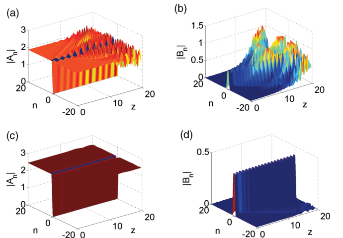
FIG. 9. (Color online) Propagation of discrete solitons for s = 1 : (a, b) \lambda = 3.5 , (c, d) \lambda = 6 . Similar behavior is obtained for s = -1 .
