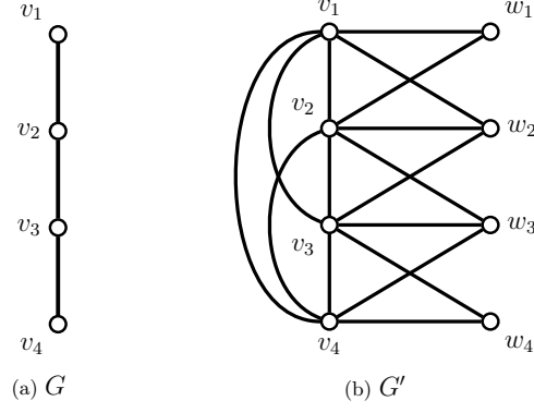
Figure 4: Example for the reduction of Theorem 4.
