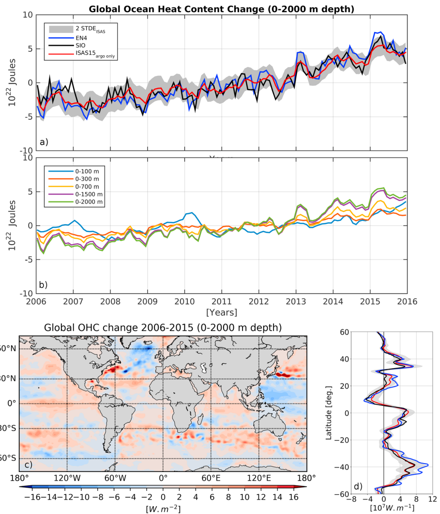
Figure 1. (a) The 0–2,000-m depth Global Ocean Heat Content Change (in J) using ISAS15 (red), Roemmich and Gilson SIO (black), EN4 (blue) along with error bar ( 2\epsilon ) computed on ISAS15. (b) Depth-layer contribution to the Global Heat Content Change in depth ranges 0–100 m (blue), 0–300 m (red), 0–700 m (yellow), 0–1,500 m (purple), and 0–2,000 m (green) depth from ISAS15. (c) The 0–2,000-m depth OHC trend over the period 2006–2015 (in W/m^2 ) from ISAS15. (d) Zonal integrated 0–2,000-m depth OHC trend over the period 2006–2015 (in W/m ) from ISAS15 (red), SIO (black), and EN4 (blue).
