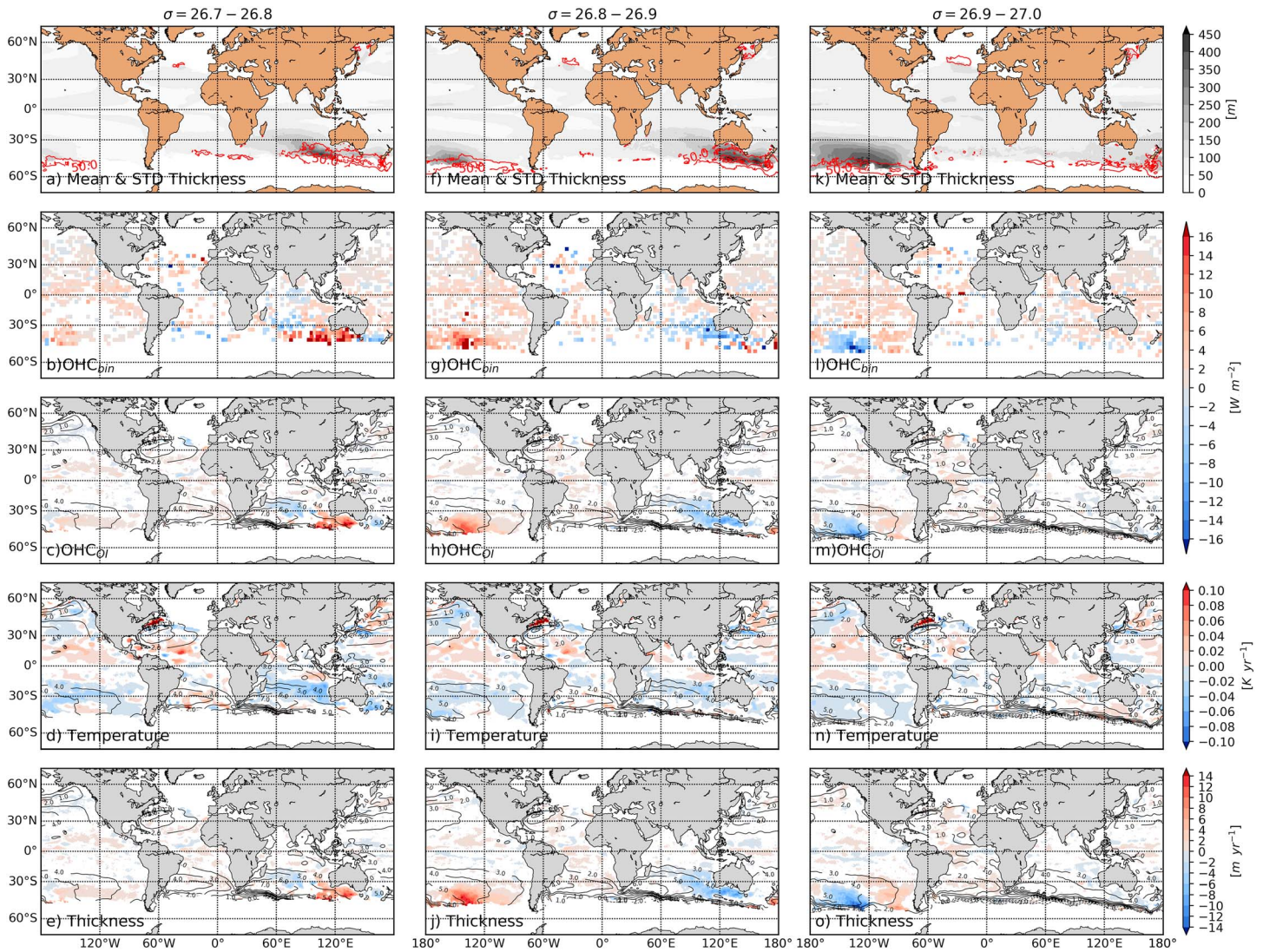
Figure 5. Same as Figure 4 except for density ranges of SAMW masses: (a–e) \sigma_\theta = 26.7\text{--}26.8 , (f–j) \sigma_\theta = 26.8\text{--}26.9 , and (k–o) \sigma_\theta = 26.9\text{--}27.0 .
