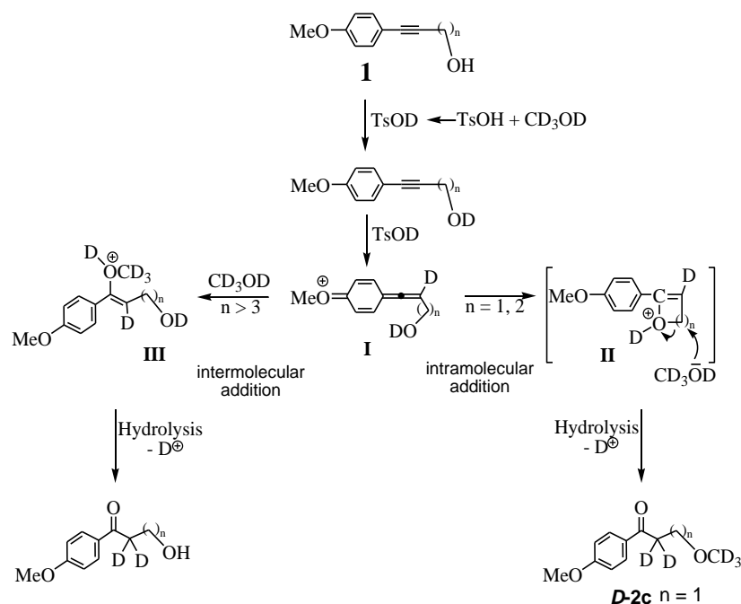
Scheme 2. Mechanism proposed for PTSA-catalyzed hydration of alkynols in \text{CD}_3\text{OD}
