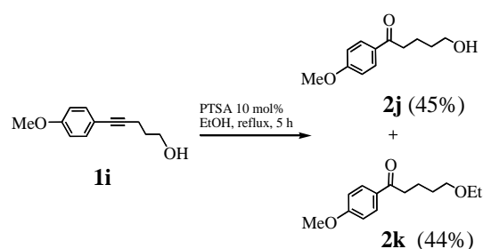
Scheme 3. Hydration of alkyne 1i
