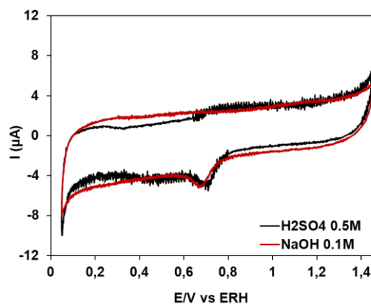
Fig. 4. Cyclic voltammograms recorded on a PdPt/C catalyst (scan rate: 10mV s -1 , N 2 saturated 0.5M H 2 SO 4 and 0.1M NaOH)
