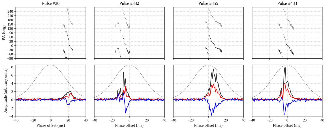
Figure 7. Polarization profiles (at 1.4 GHz) of four example single pulses showing a smooth and uninterrupted 180-deg sweep of the PA at different phases . The time resolution of the data is 740 \mu s. Top panel: phase-resolved PA (black points) where the data are repeated a second time with a shift of 180 deg (grey points) for readability. Bottom panel: polarization profiles, with total intensity in black, linearly and circularly polarized flux in red and blue, respectively. The grey dashed line represents the best-fitting Gaussian to the integrated pulse intensity over the whole observation. Such continuous 180-deg rotation of the PA is somewhat reminiscent of the rotating vector model prediction for an inner line of sight (see text). However, the fact that the sweep occurs at different phases in every pulse is remarkable and difficult to explain. This behaviour is visible in a dozen pulses in the 2-h observation.
