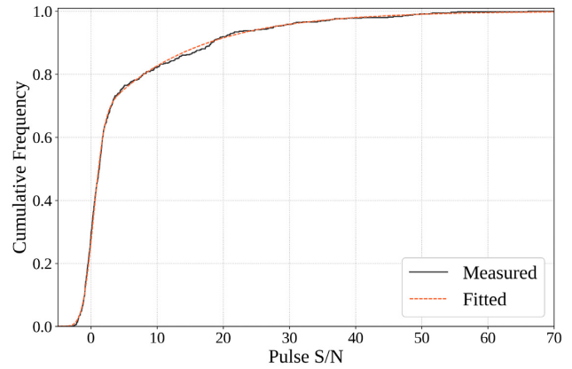
Figure 6. Cumulative distribution function of single pulse energies measured on the 2-h main observation (solid black line). S/N values are the integrated intensities of every pulse over an identical phase window, divided by the appropriate normalization factor. The intrinsic pulse energy distribution is well fitted by an exponential distribution modulated by a nulling probability of 65 per cent (dashed orange line).
