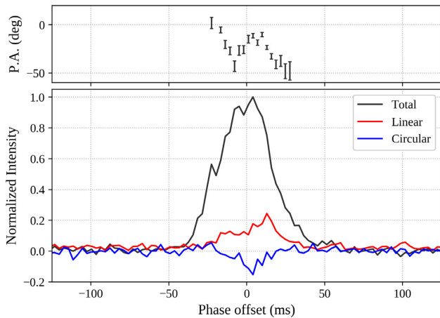
Figure 4. Bottom panel: mean polarization profiles at 1382 MHz, normalized to peak total intensity and corrected for Faraday rotation. Top panel: PA of the linearly polarized flux. Phase offset is measured from the peak of the Gaussian fit to the mean pulse intensity.
