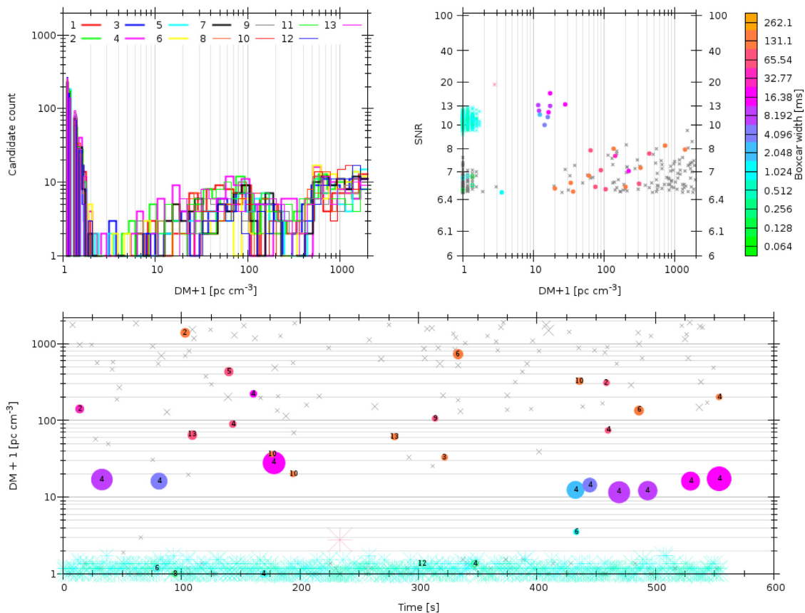
Figure 1. Discovery plot of PSR J2251–3711 as produced by the HEIMDALL single pulse search pipeline. Detected pulses in this 9-min discovery observation are shown as filled circles in the bottom panel in a time–dispersion measure (DM) diagram. The colour denotes the value of the best-fitting pulse width, and the circle size indicates signal-to-noise ratio (SNR). The beam number in which they were detected is overlaid. Top left: DM distributions of detected single pulses, plotted for every individual beam. Top right: detected single pulses in a DM–SNR diagram, for all 13 beams of the receiver.
