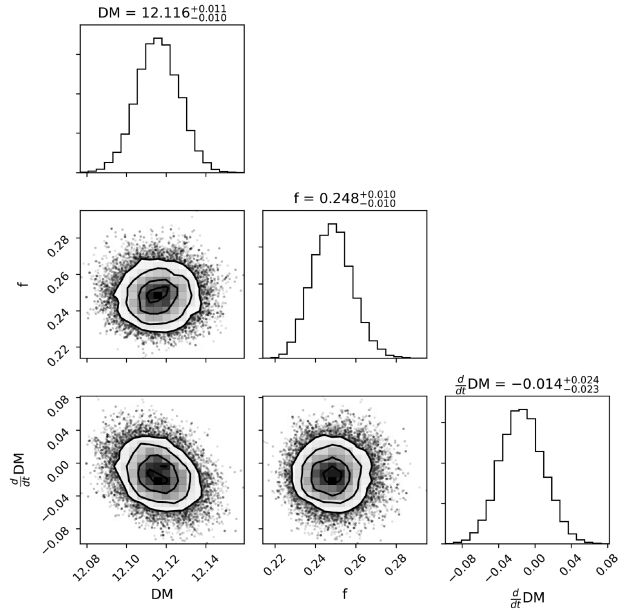
Figure 2. Posterior probability densities for the source DM, DM rate of change (here in \text{pc cm}^{-3} \text{ yr}^{-1} ), and the dimensionless DM uncertainty scale factor f (see equation 1 and text for details). They were fitted to a sample of 326 single pulses detected by the search pipeline HEIMDALL across all Parkes multibeam observations of PSR J2251–3711. The lower and upper uncertainties quoted for all parameters correspond respectively to the 16th and 84th percentiles of their probability distributions.
