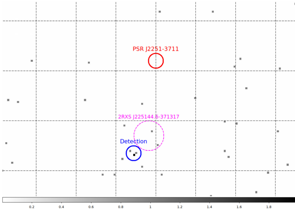
Figure 8. Swift X-ray image of the field, with a total exposure time of 4.4 ks. Only a zoom on the region of interest is shown. The coordinate grid spacing is 1 arcmin on both RA (horizontal) and Dec. (vertical) axes. Red circle: half power diameter (18 arcsec) of the Swift PSF centred on the radio timing position of PSR J2251–3711, enclosing zero counts. Blue circle: a 4-count detection with a statistical significance of 4.5\sigma . Magenta dashed circle: the 1\sigma position uncertainty on the original detection of the ROSAT faint source 2RXS J225144.6–371317.
