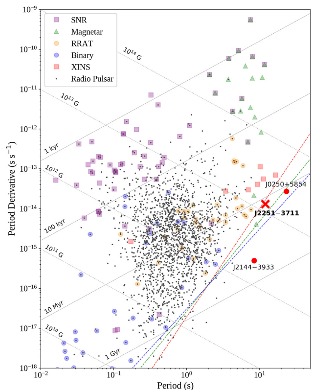
Figure 3. P - \dot{P} diagram, based on v1.59 of the ATNF pulsar catalogue (Manchester et al. 2005). The period and period derivative ranges on the plot have been set to concentrate on the non-recycled pulsar population. The radio pulsars with the three longest spin periods have been highlighted in red. Lines of constant characteristic age and surface magnetic field strength are displayed in grey. The dashed red line represents the lower limit of the so-called pulsar death valley (equation 8 of Chen & Ruderman 1993). Death lines from Zhang et al. (2000) are also shown, based on their curvature radiation from vacuum gap model (green dashes) and space-charged-limited flow model (blue dashes).
