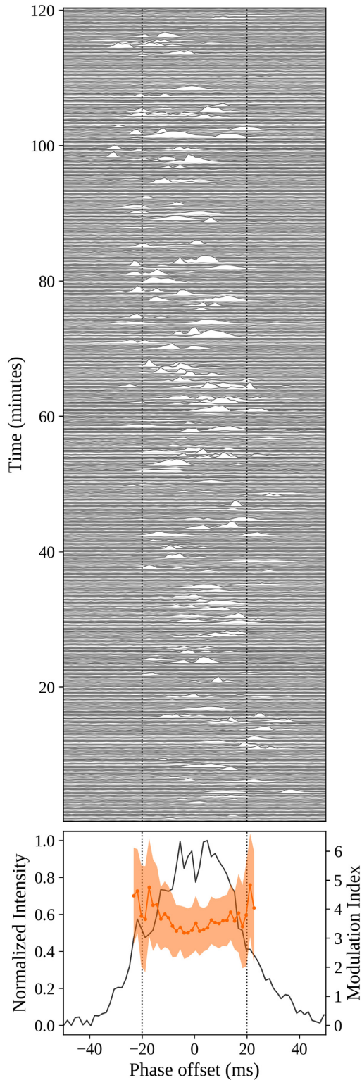
Figure 5. Top panel: single pulses from a continuous 2-h observation at a centre frequency of 1382 MHz. The vertical lines denote the FWHM of the Gaussian pulse fit. Bottom panel: Phase-resolved flux density (grey line, left axis) and modulation index (orange points, right axis) around the on-pulse region. The 1\sigma errors are represented by the shaded area. The overall tendency of single pulses to arrive earlier as the observation progresses is statistically significant (see text), and could be evidence for the presence of drifting sub-pulses tracks, wrapping around in phase on a time-scale of several hours.
