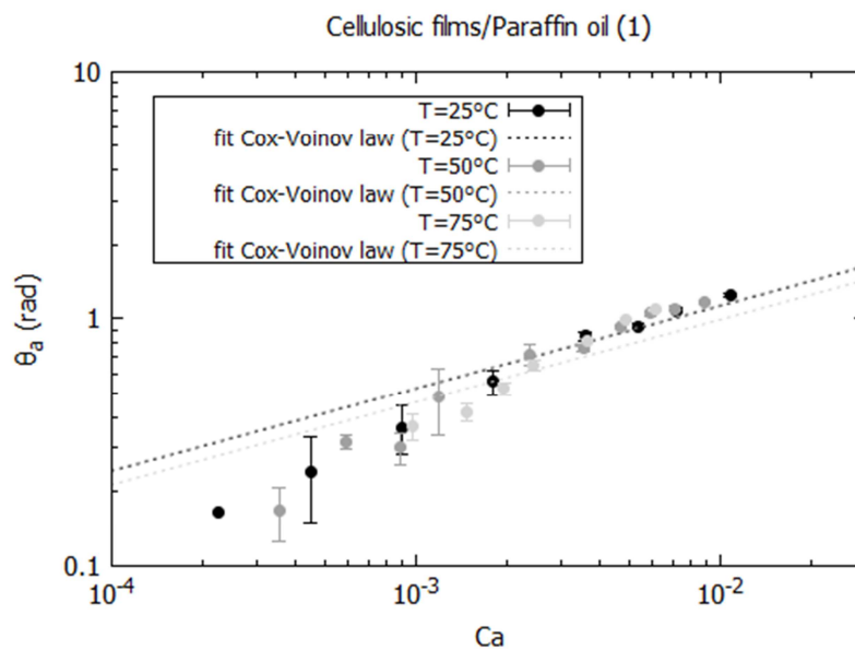
Figure 2: Advancing contact angles as a function of capillary number and fits according to the Cox-Voinov law.
