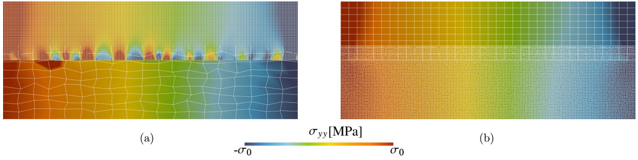
Figure 18: Bending stresses \sigma_{yy} : (a) Case 1, (b) Case 2.
