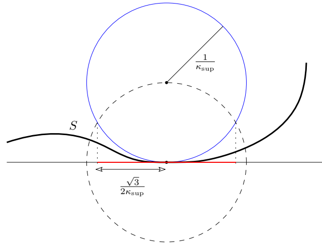
■ Figure 1 Illustration of the proof of Lemma 3.1 for the 2D case.
