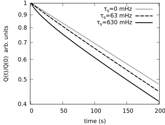
Figure 4: Discharge curves Q(t) for three different surface relaxation rates namely \tau_s = 0 (grey full line), \tau_s = 63 mHz (dashed black line), \tau_s = 630 mHz (black full line). The percentage of the amount of charge that decays via both channels was fixed to 20% ( Q_c(0)/Q(0) = 0.2 ).
