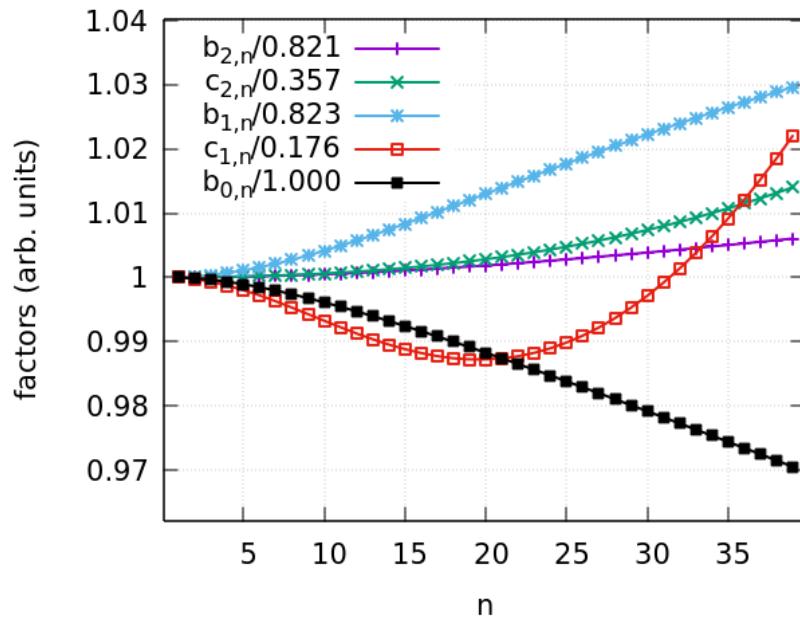
Figure 1: Relative variation of the factors as a function of n
