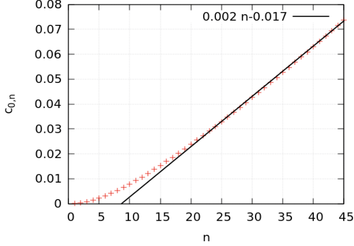
Figure 2: Dependence of the factors c_{0,n} on the integer n
