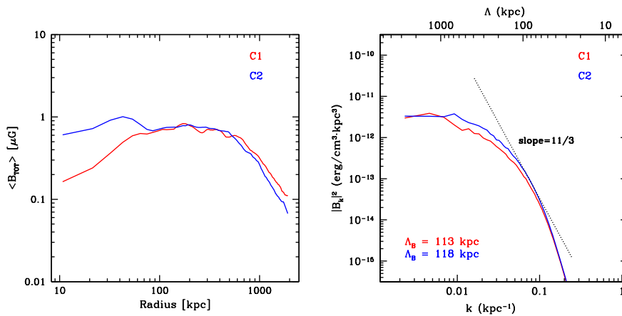
Figure 2. Left: average of the total magnetic field 3D profiles for the C1 (red) and C2 (blue) clusters. Right: magnetic field power spectra for the C1 (red) and C2 (blue) clusters. The autocorrelation length values are shown in the bottom left corner. A dotted black line shows a power spectrum with spectral index equal to 11/3.
