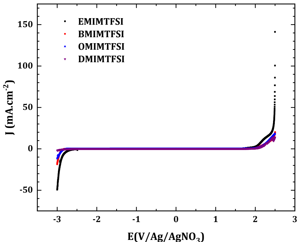
Figure 4- Linear sweep voltammeteries on gold electrode for the four RTILs at 5 \text{ mV.s}^{-1} at 298K
