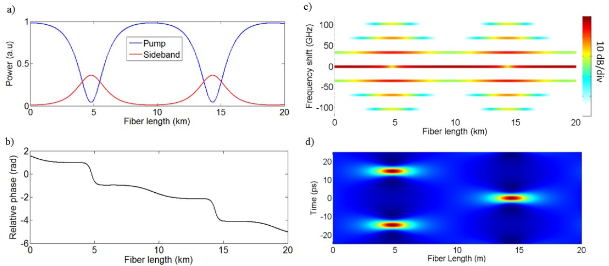
Fig. 1. Longitudinal evolution of (a) the normalized pump and sideband powers and (b) the pump-sideband relative phase. (c) and (d) shows the spectral and the temporal evolution of the intensity along the fibre, respectively. Parameters: fibre length L = 20 km, \beta_2 = -19 \times 10^{-27} \text{ s}^2/\text{m} , \gamma = 1.3 \times 10^{-3} \text{ /W/m} , P_p = 450 \text{ mW} , sideband to pump ratio \eta = 0.01 , sideband detuning 35 GHz. Powers are normalized to their maximum values.
